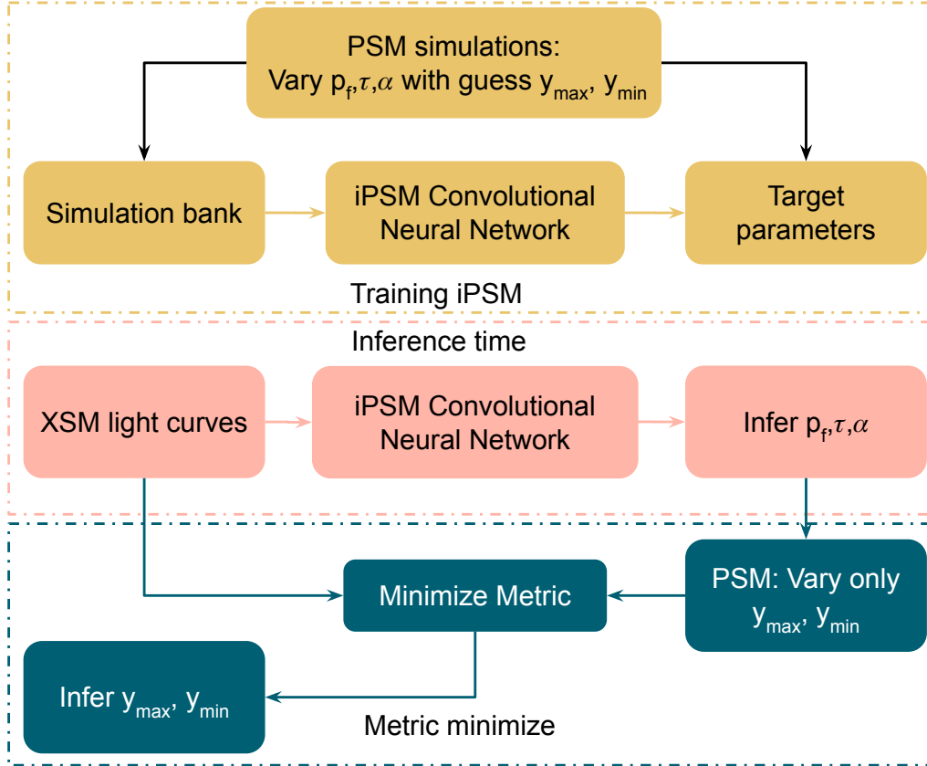
Figure 2. Flow chart detailing the various steps in our algorithm. First, the iPSM is trained on simulations. Next, the trained model is used to infer p_f , \tau and \alpha . Finally, the y_{max} and y_{min} are inferred by minimizing an error metric.
