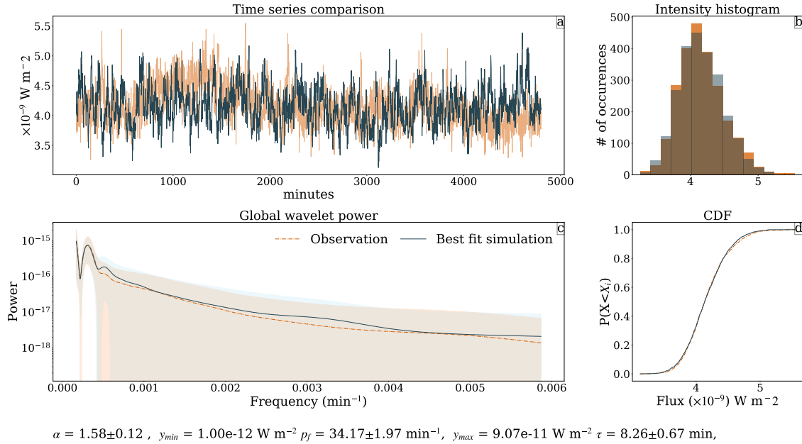
Figure 4. Comparison of the observed light curve from XSM (orange), and the PSM forward model of best fit parameters inferred from our inversion code (black) in 1-2.3 keV energy band from 2019 (sub figure: I) and 2020 (sub figure: II). Each sub-figure has four panels depicting: Panel (a): Observed and simulated light curves; Panel (b): Distribution of observed and simulated light curve intensities; Panel (c): Global Morlet power for observation and simulations, with the uncertainties presented in orange and blue bands; Panel (d): Comparison of simulation and observation intensity CDF. The inset reports the inferred parameter set for the respective data.
