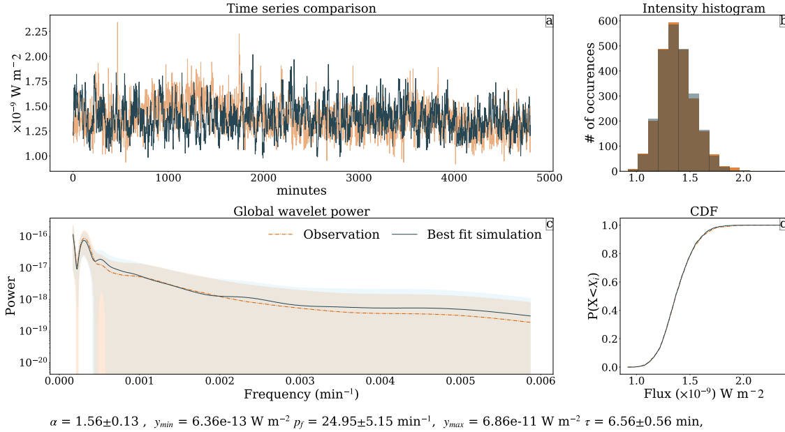
Figure 6. Same as Fig. 4, but for 1.3–2.3 keV band for the segment from year 2020.
