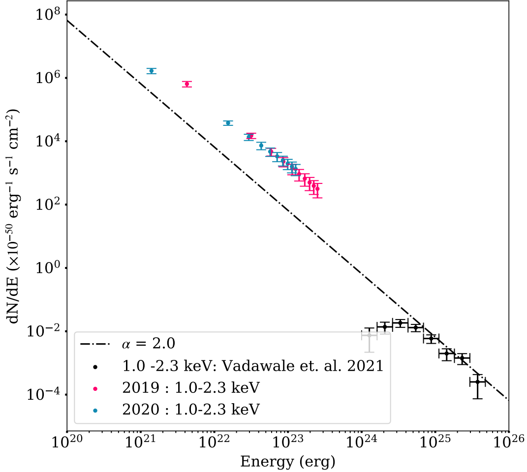
Figure 7. Frequency distribution of impulsive events inferred from the observations in 2019 year (pink) and 2020 (cyan). The scatter is frequency distribution of event energies from the model. The errorbars on inferred parameters are obtained by propagating the Monte Carlo uncertainties. The black scatter shows the inferred frequency distribution from Vadawale et al. (2021b) , while the black dot-dashed line corresponds to \alpha = 2.0 .
