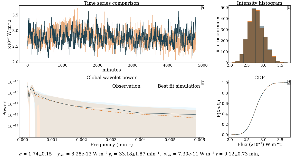
Figure 5. Same as Fig. 4, but for 1.3–2.3 keV band.
