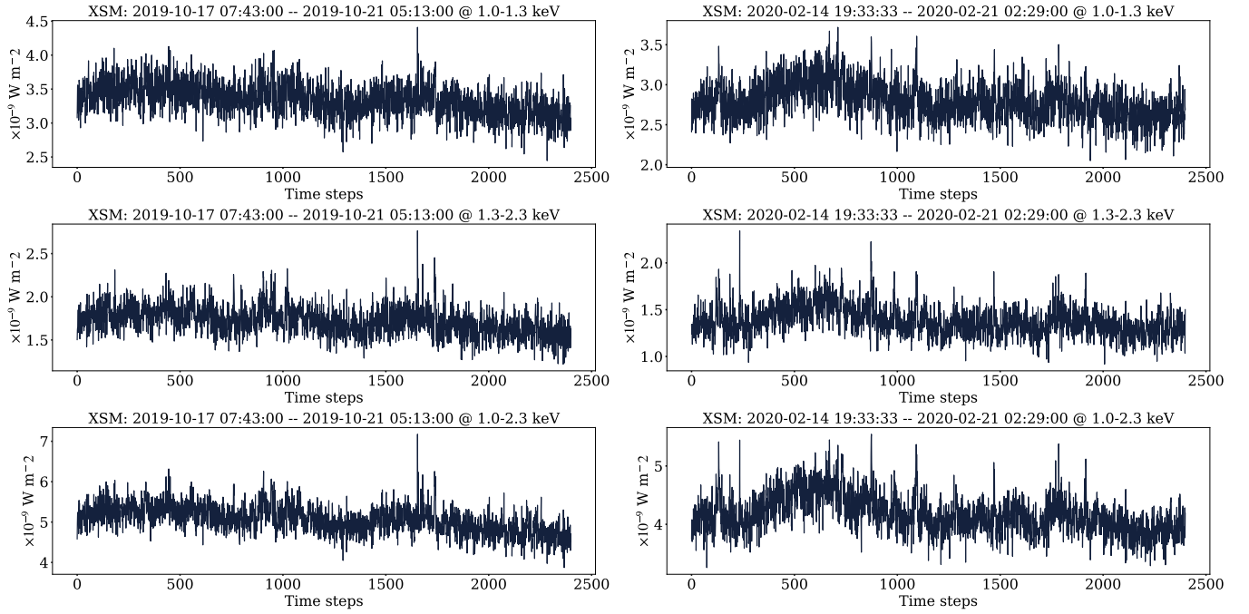
Figure 1. The XSM observed light curves considered in this work. The left(right) column is for 2019(2020) observations. Top row is the light curve for 1.0–1.3 keV, middle row is for 1.3–2.3 keV and the bottom row is for 1.0–2.3 keV.
